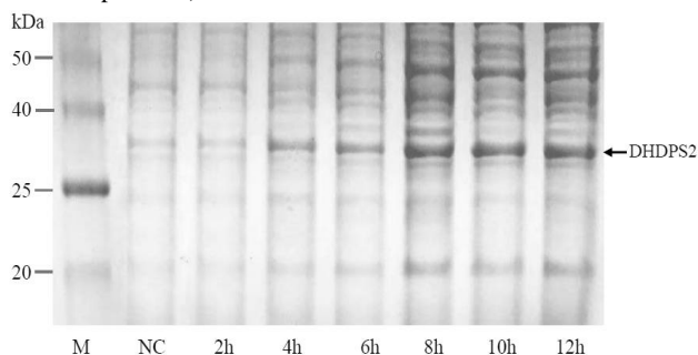
Fig 5: SDS-PAGE analysis of the expression of recombinant DHDPS2 protein in E. coli . BL21 (DE3) cells on YJ culture medium. M: protein weight marker, NC: without IPTG. Other lanes: with 0.5 mM IPTG at 2, 4, 6, 8, 10, 12 h, respectively.
