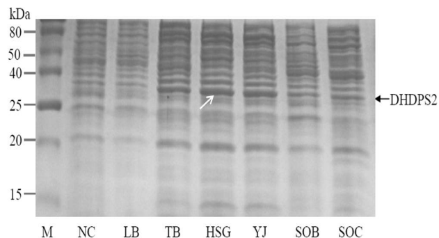
Fig 7: SDS-PAGE analysis of the expression of recombinant DHDPS2 protein in E. coli . BL21 (DE3) cells in different culture mediums. M: protein weight marker, NC: transformed E. coli cells on YJ culture medium without IPTG induction. Other lanes: culture mediums of LB, TB, HSG, YJ, SOB, SOC with 0.5 mM IPTG induction, respectively.
