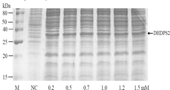
Fig 6: SDS-PAGE analysis of the expression of recombinant DHDPS2 protein in E. coli . BL21 (DE3) cells on HSG culture medium with different concentrations of IPTG induction at 8h. M: protein weight marker, NC: without IPTG. Other lanes: with IPTG at 0.2, 0.5, 0.7, 1.0, 1.2 and 1.5 mM, respectively.
