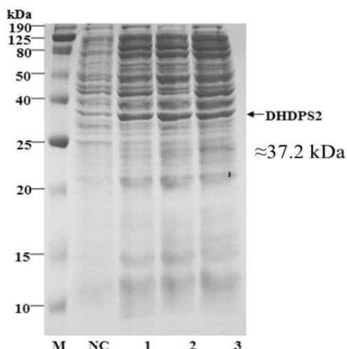
Fig 4: SDS-PAGE analysis of the expression of recombinant DHDPS2 polypeptides in E. coli . BL21 (DE3) cells on YJ culture medium. M: protein weight marker (10-190 kDa, Bioline), NC: transformed E. coli cells without IPTG induction. Lanes 1, 2, 3: transform which designed to base on the coding DNA sequence (CDS) for the mature peptide of E. coli cells with 0.5 mM IPTG induction (three times replicative).
