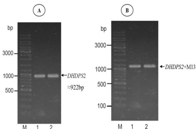
Fig 1: PCR amplification of the mature peptide coding sequence of DHDPS gene (accession no: XM_01358955.2) from genomic DNA of M. truncatula . M: DNA size marker (100-10000 bp, GeneRuler™ DNA Ladder), 1 (A): PCR product of DHDPS-F/DHDPS-R specific primer pair, 1 (B): PCR product of M13 primer pair of pGEM@-T Easy vector.
