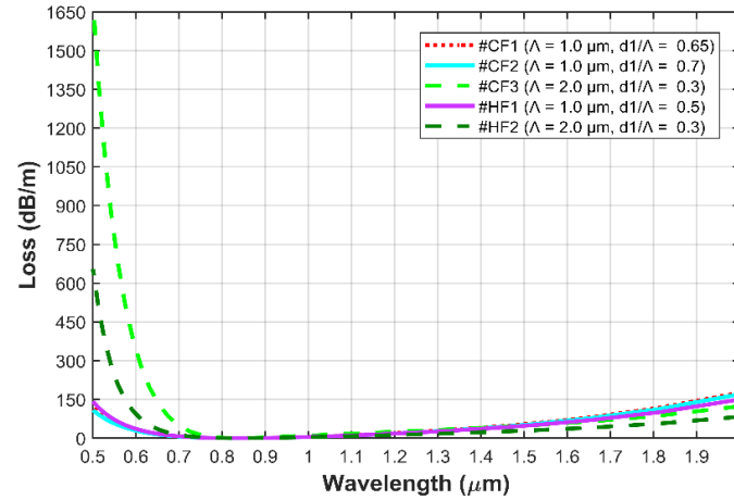
Figure 5: The confinement loss of optimal PCFs for the circular lattice and hexagonal lattice
