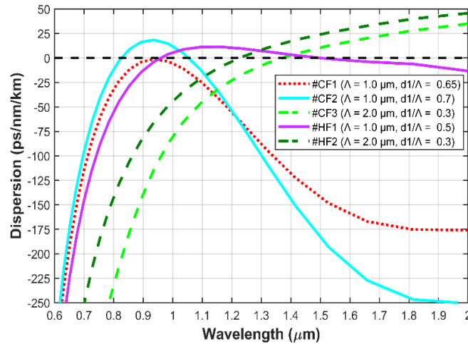
Figure 2: The optimal dispersion curves synthesis of circular and hexagonal lattices PCFs infiltrated with \text{CHCl}_3
