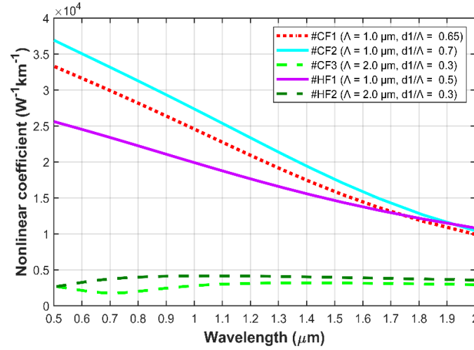
Figure 4: The nonlinear coefficients of #CF 1 , #CF 2 , #CF 3 , #HF 1 , and #HF 2 fibers
