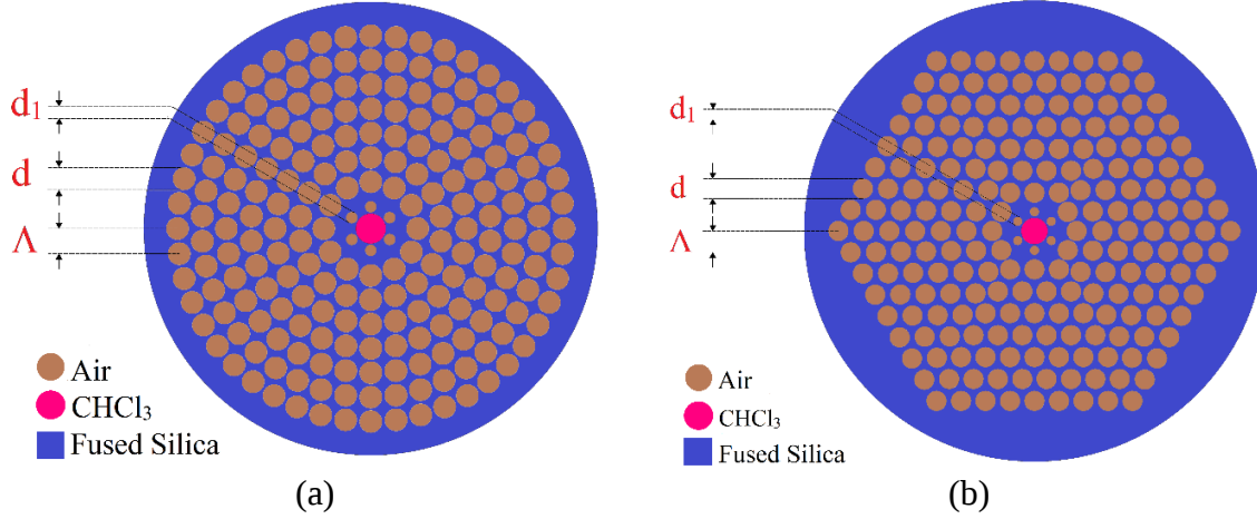
Figure 1: The geometrical structure of PCF with the circular lattice (a) and hexagonal lattice (b)
