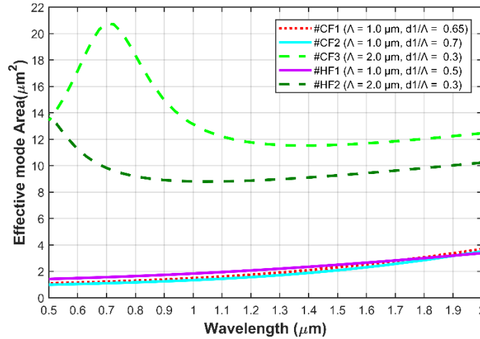
Figure 3: The effective mode area of optimal PCFs for circular and hexagonal lattices
