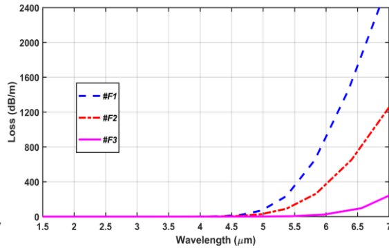
Figure 7: Confinement loss characteristics of the proposed PCFs
