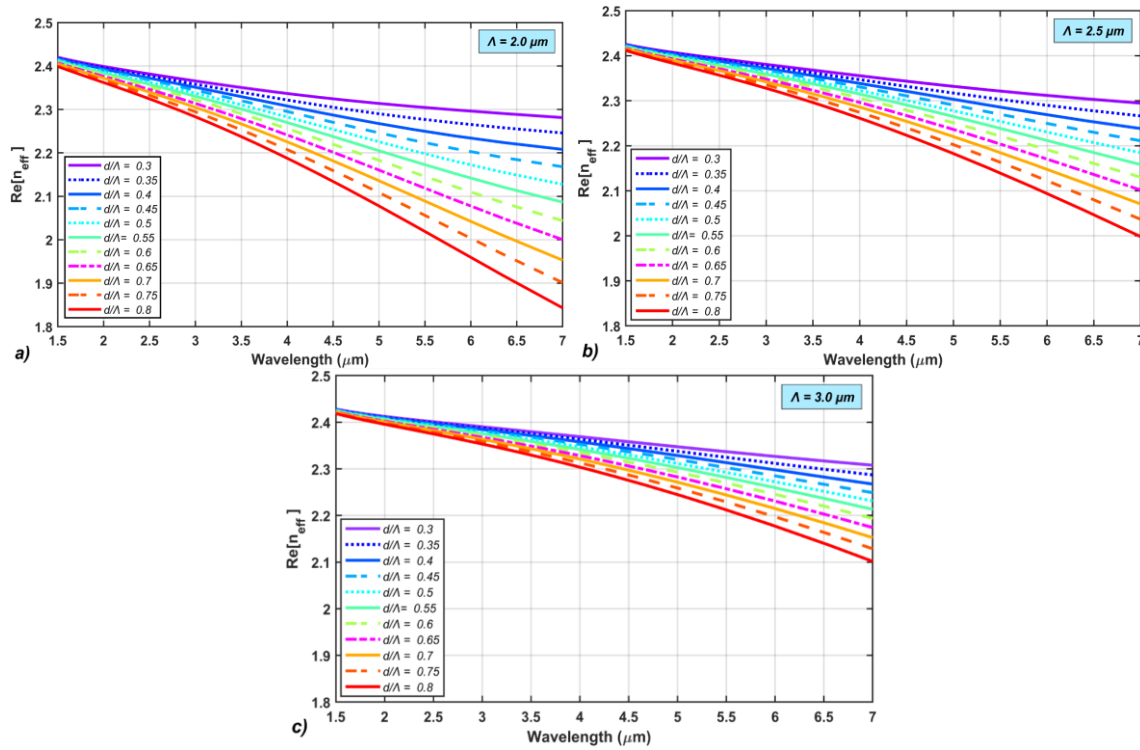
Figure 2: The real part of effective refractive index depend the wavelength of PCF with various d/\Lambda for the cases of a) \Lambda = 2.0 \mu\text{m} , b) \Lambda = 2.5 \mu\text{m} and c) \Lambda = 3.0 \mu\text{m}
