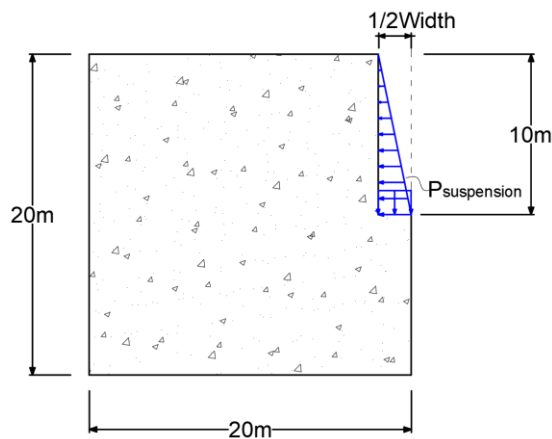
Figure 3. The model dimensions of the bentonite suspension trench in 2D.
