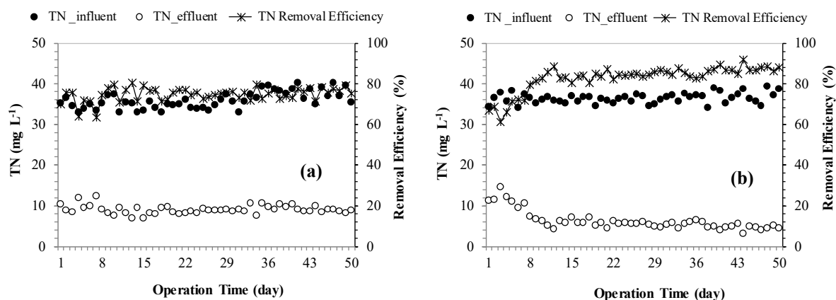
Fig. 7 Total nitrogen (TN) removal efficiency in R1 (a) and R2 (b) during operation time
