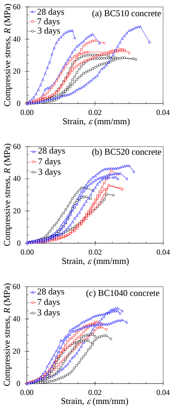
Fig. 9. Compressive stress-strain relationships of SS concretes
