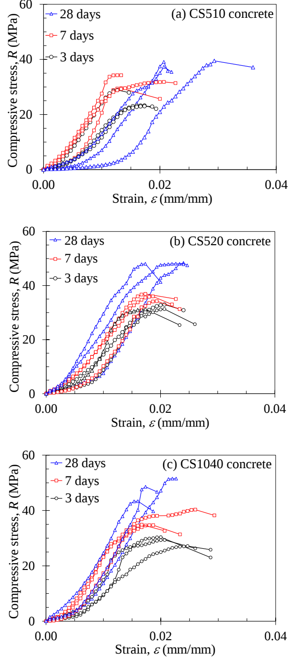
Fig. 10. Compressive stress-strain relationships of CS concretes
