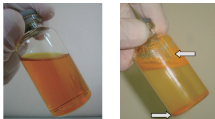
(a) (b) Solubility of (a) Cur-Glu and (b) Cur in water.
